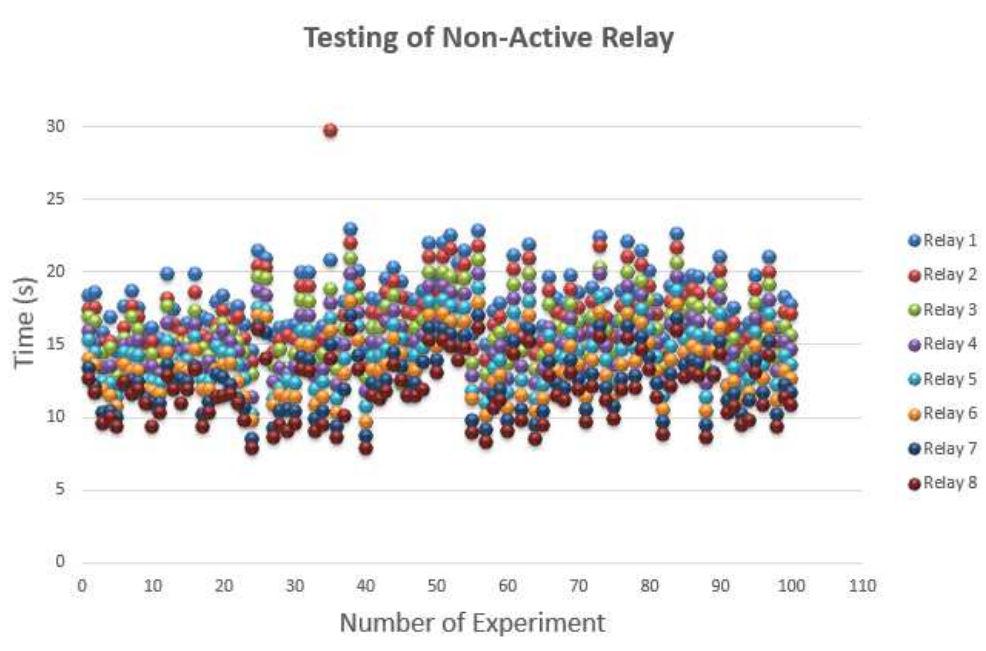
Figure 6. Non-Active Time Testing of Relay in 100 Experiment
