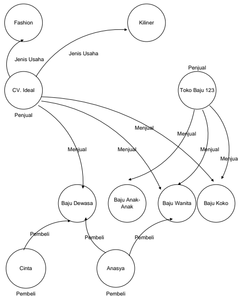
Gambar 2 Rancangan Basis Data Graph
