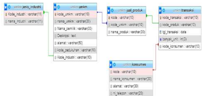
Gambar 1 Basis Data Relasional
